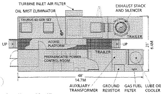
Installation Plan View
